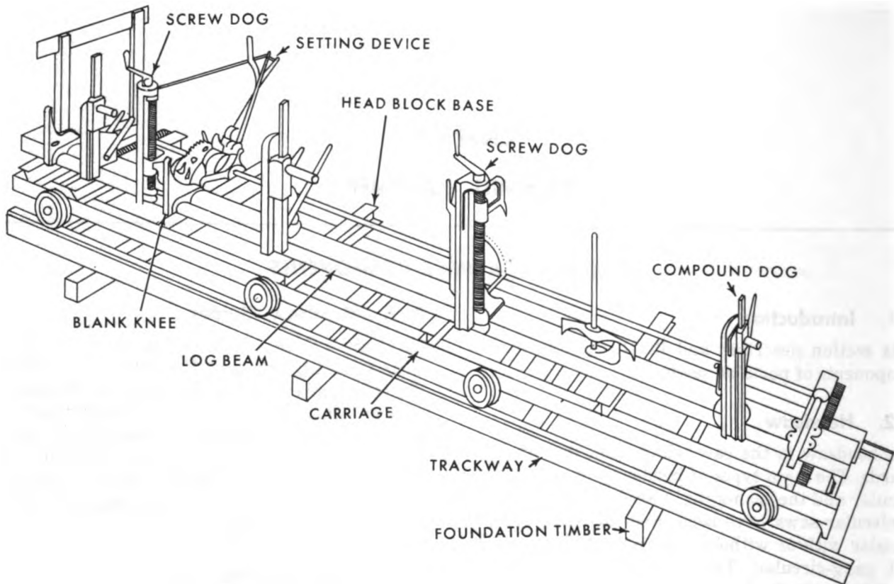
Figure 8-2. Log-beam type carriage.
